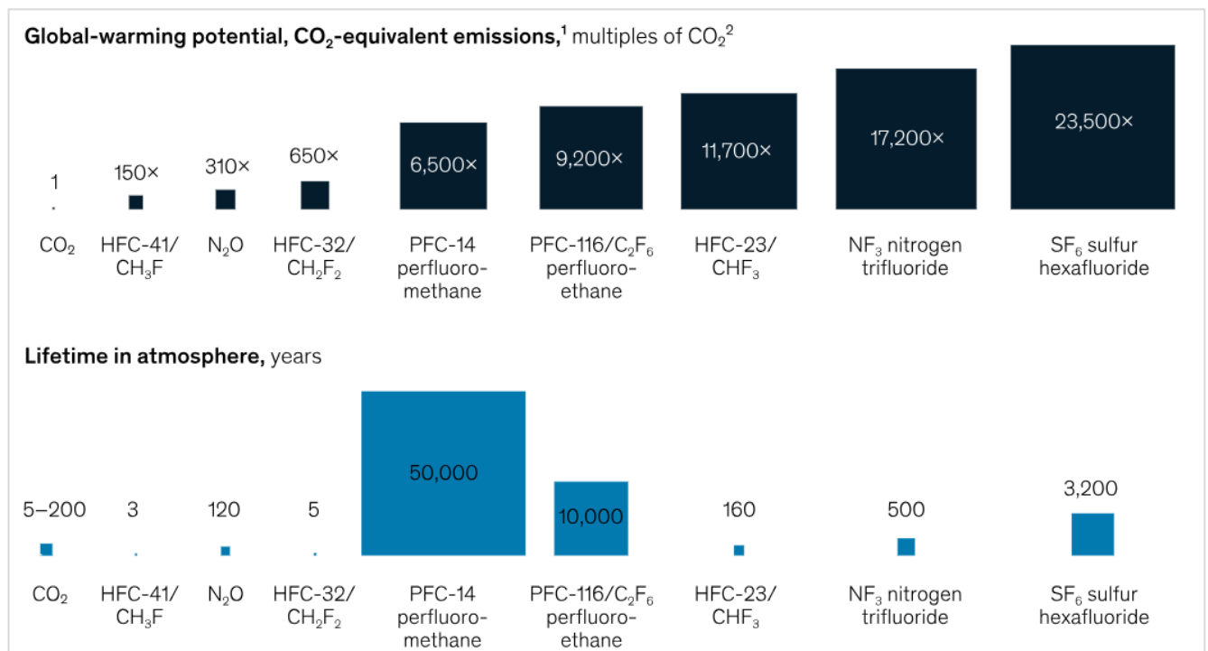
Figure 17: Environmental impact of semiconductor manufacturing process gases [31].
